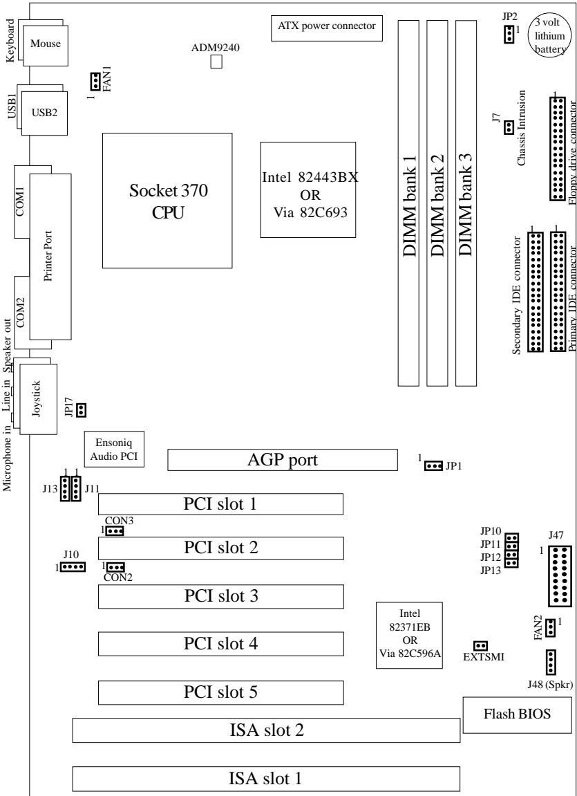
Figure 2-3 : Map of Motherboard Jumpers
