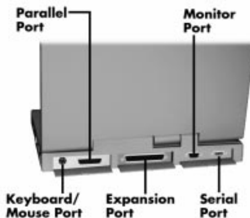
Figure 2-3 Power and I/O Connector Locations
