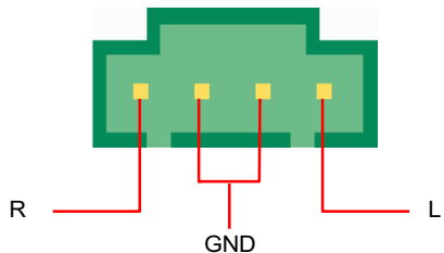
MODEM-IN
