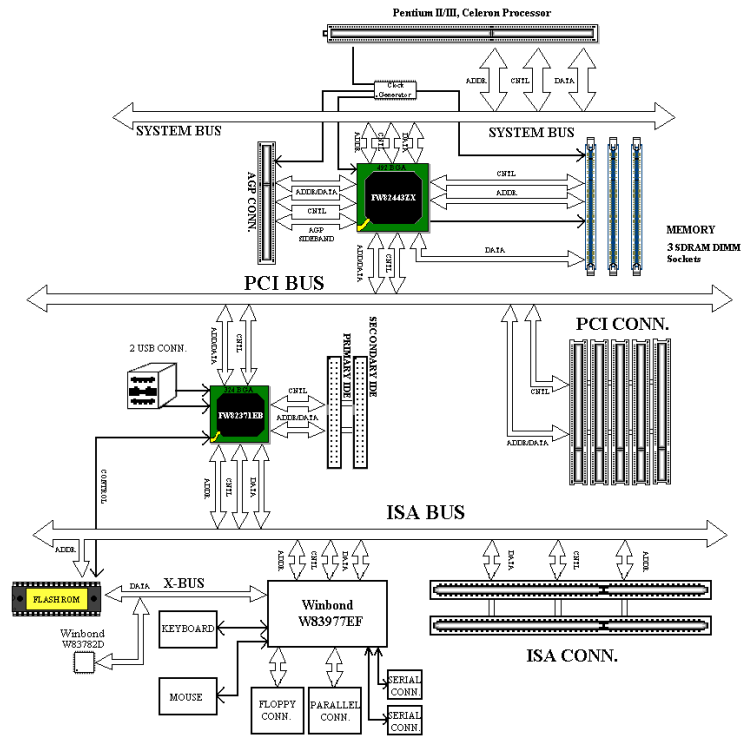
Figure 1-3. System diagram of the 440ZX chipset
