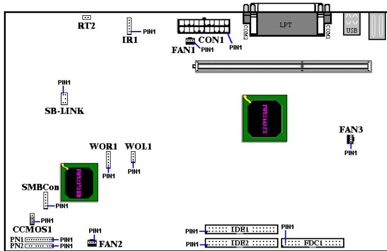
Figure 2-5. All Connectors and Headers for the ZH6
