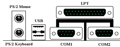
Figure 2-11. ZH6 back panel connectors
