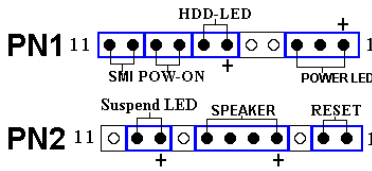
Figure 2-9. The definition of PN1 and PN2 pins
