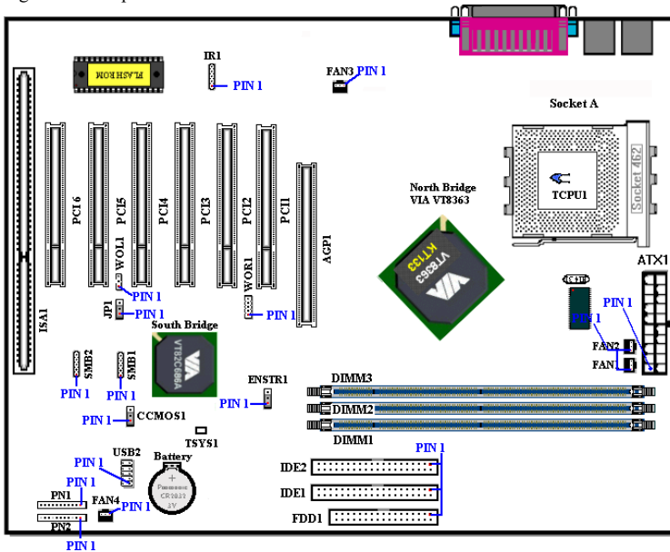
Figure 2-7A. All Connectors and Headers for the KT7
