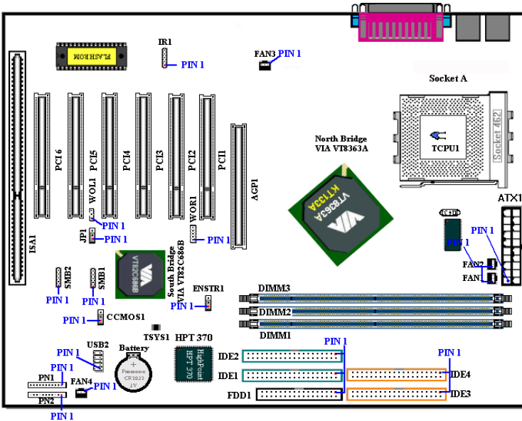
Figure 2-7D. All Connectors and Headers for the KT7A-RAID
