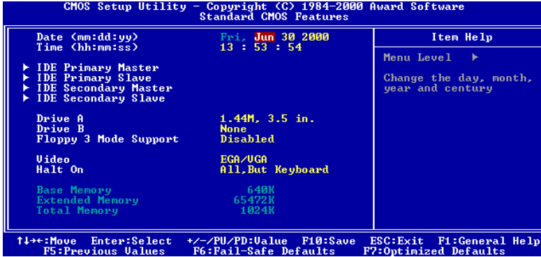
Figure 3-3A. Standard CMOS Setup Screen Shot
