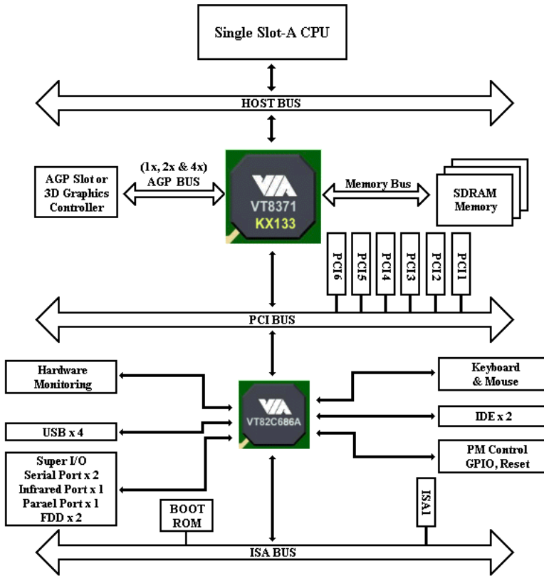
Figure 1-3. System diagram of the KA7
