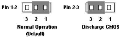
Figure 2-6. CCMOS jumper setting
