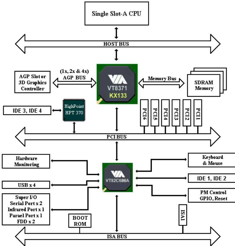
Figure 1-4. System diagram of the KA7-100
