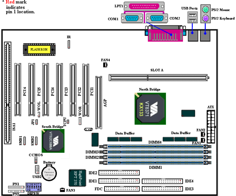
Figure 1-2. KA7-100 Motherboard component location
