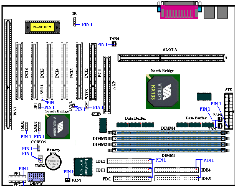
Figure 2-5A. All Connectors and Headers for the KA7-100
