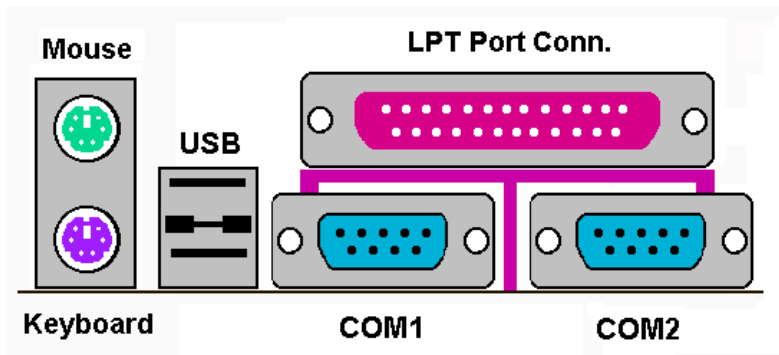
Figure 2-11. KA7/KA7-100 back panel connectors
