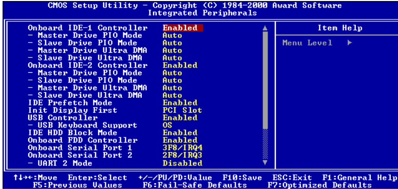
Figure 3-6A. Integrated Peripherals Menu Default Screen (KA7)
