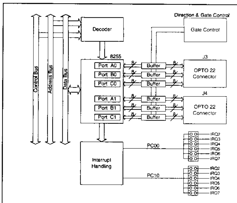
PCM-3724 Block Diagram
