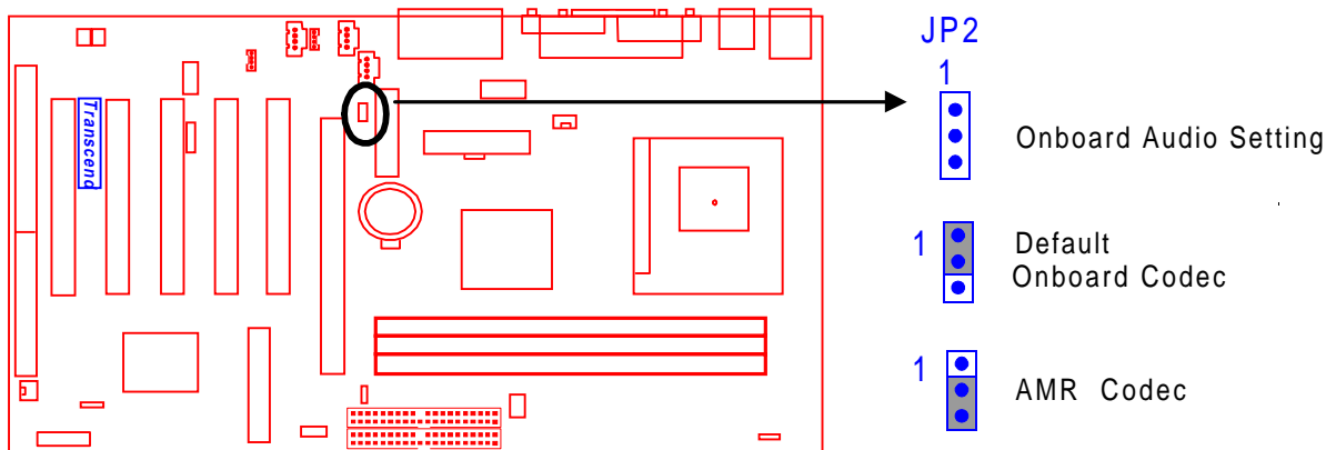
Audio Selection Jumper
