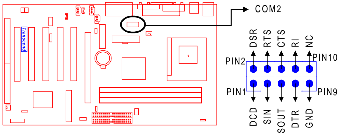
Internal Serial Port Connector COM2
