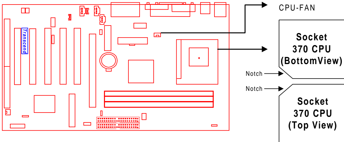
Socket 370 CPU Installation
