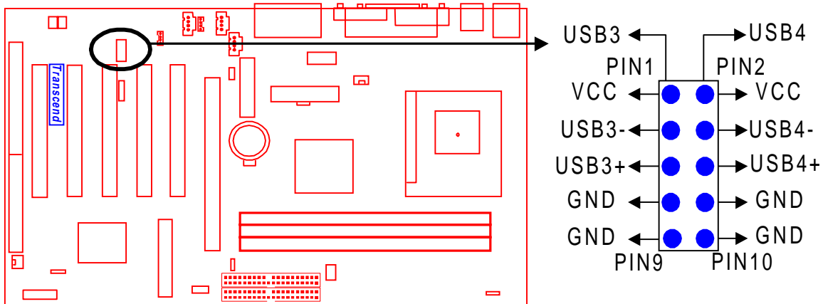
Internal USB Port Connector
