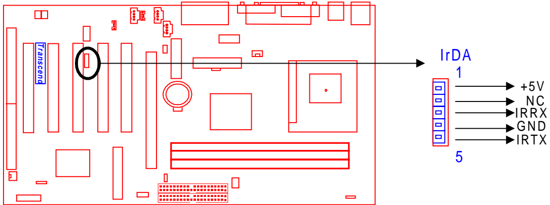
IrDA Connector
