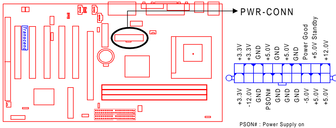
Power Connector
