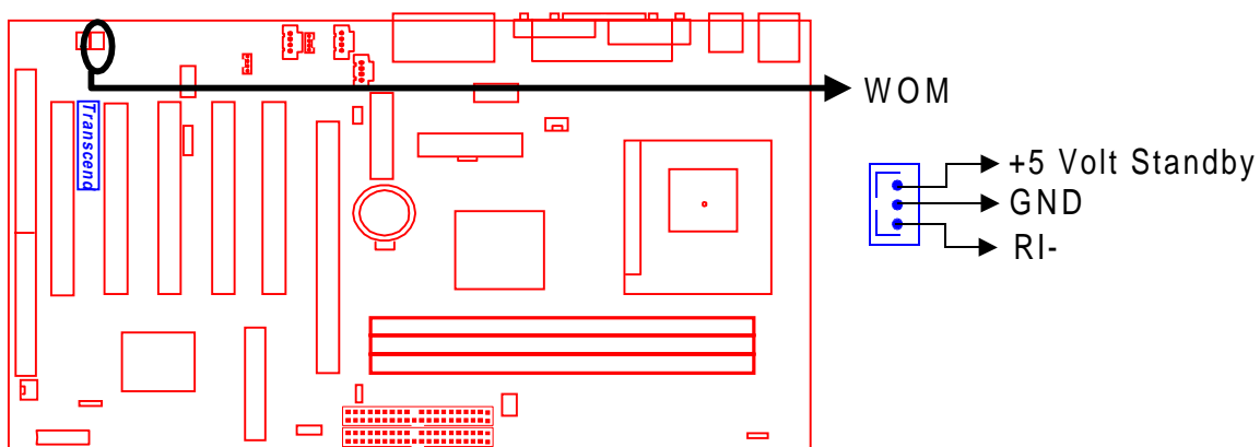
Wake-On-Modem Connector
