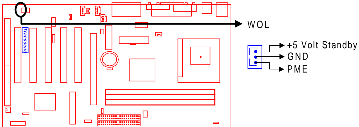
Wake-On-LAN Connector
