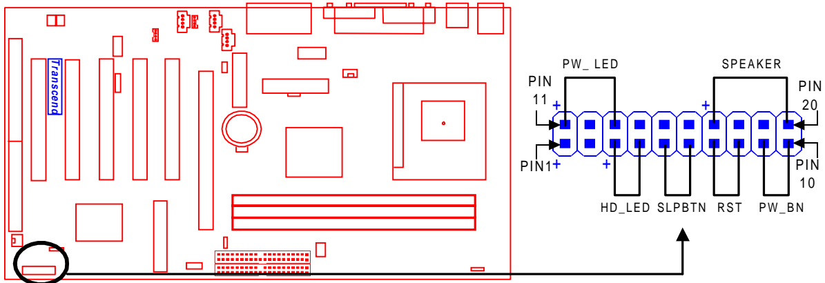
Panel Connectors
