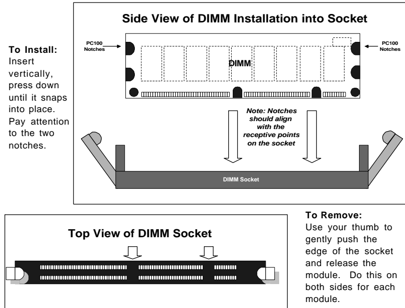
Figure 2-3. Installing the DIMM
