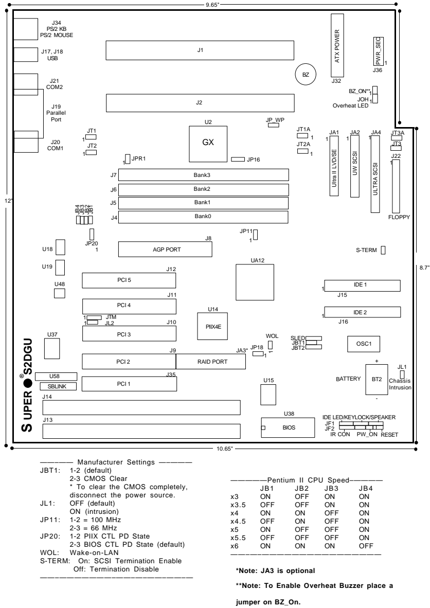
Figure 1-3. SUPER S2DGR Motherboard Layout
