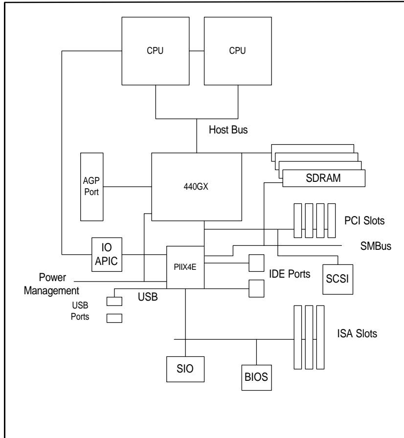
Figure 1-5. 440GX AGP SET: System Block Diagram (Dual Processors)
