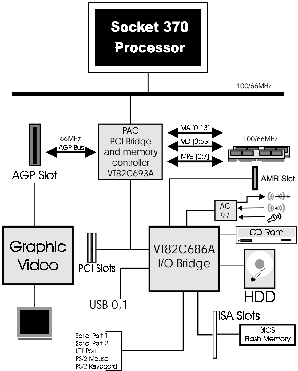
Figure 4: System Block Diagram
