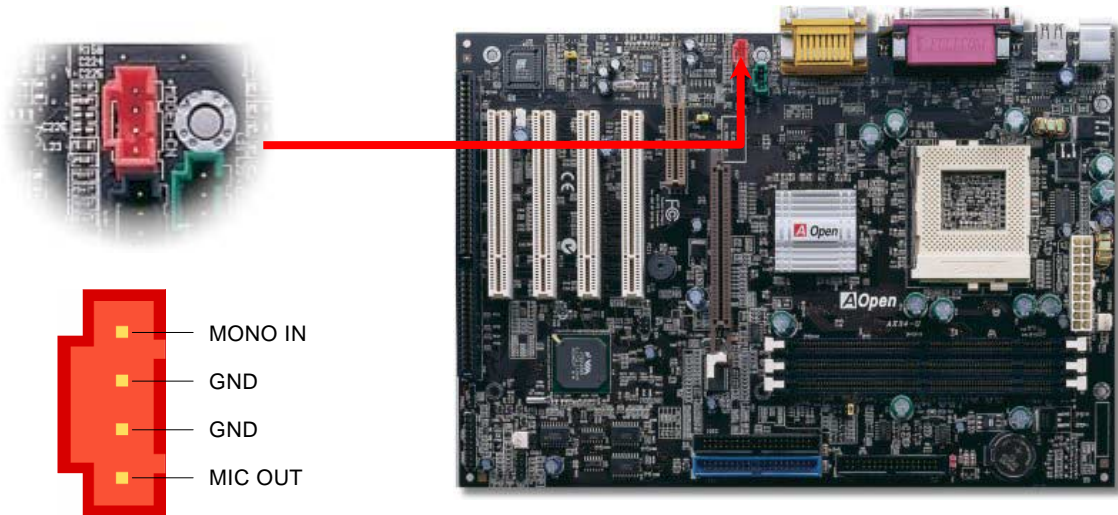
MODEM-CN Connector
