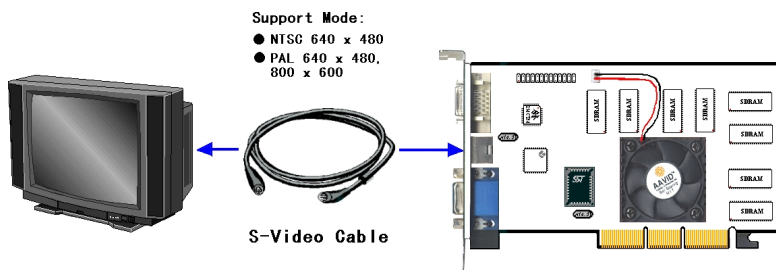
Figure 2-7. SILURO GT2V/SILURO GT2 Ultra connection to TV
