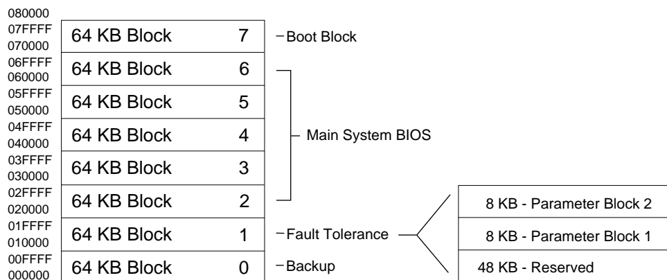
Figure 15. Memory Map of the Flash Memory Device
