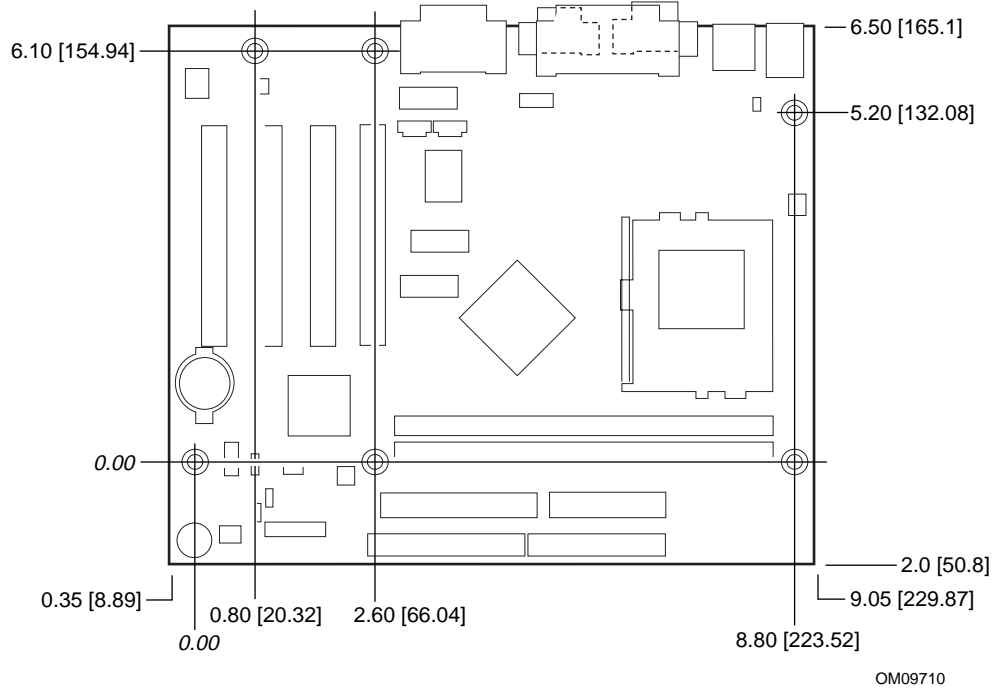
Figure 12. Board Dimensions
