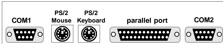
Figure 3-2: P55-KTI/O back panel Layout
