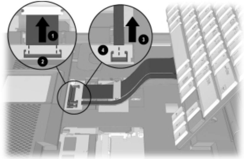
Figure 5-9. Releasing and Disconnecting the Keyboard Cables
