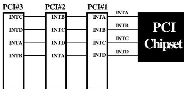
Figure 3-7 The Combination of PCIINT# lines
