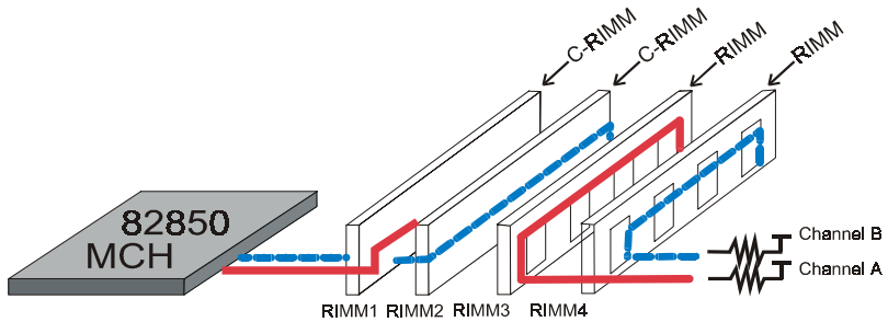
Figure 11-2: Right Base Configuration
