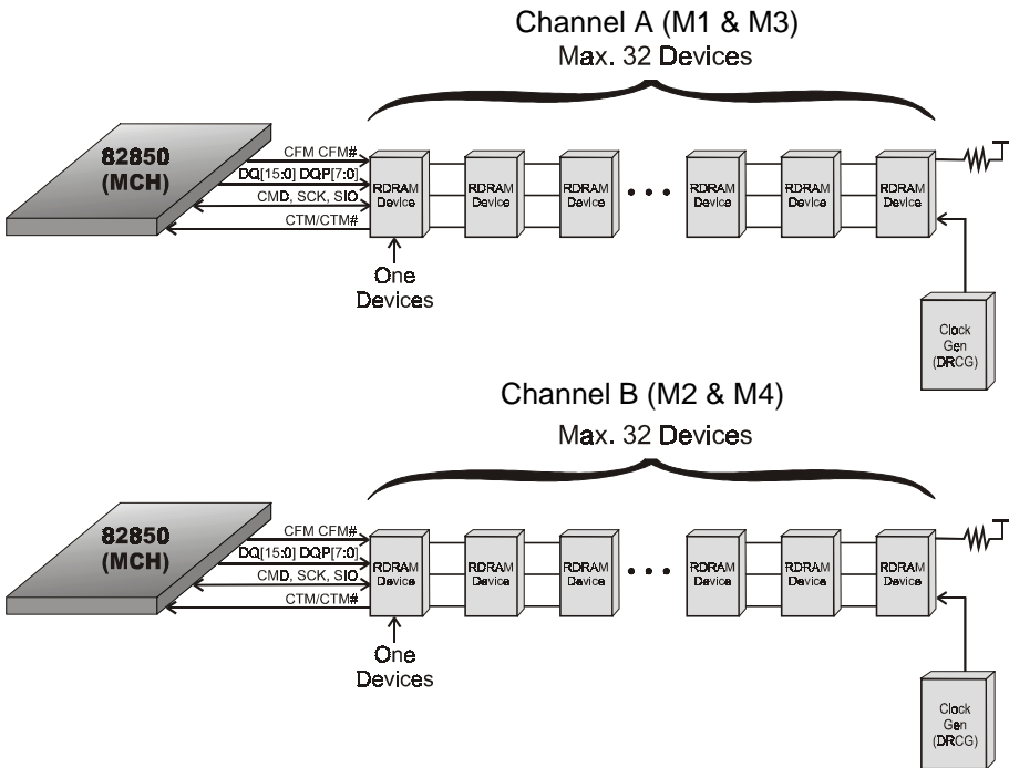
Figure 8: MCH/RDRAM Interconnections
