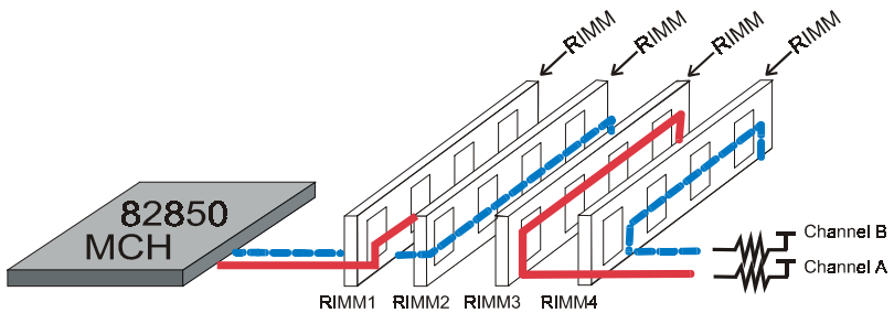
Figure 12: Right Base Configuration
