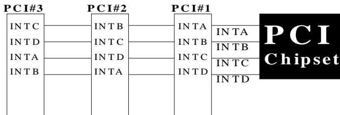
Figure 7: The Combination of PCI INT#lines
