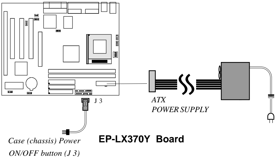
Figure 4: Simple ATX Power ON/OFF Controller
