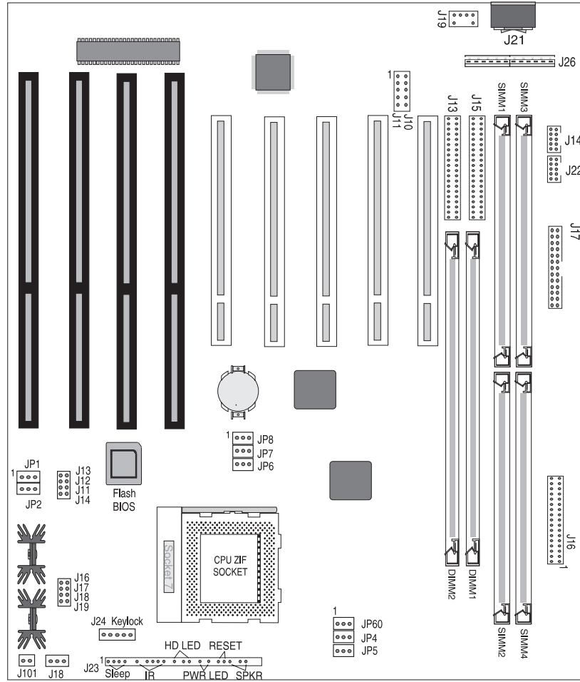
Figure 2-1. Twister AT System Board Diagram
