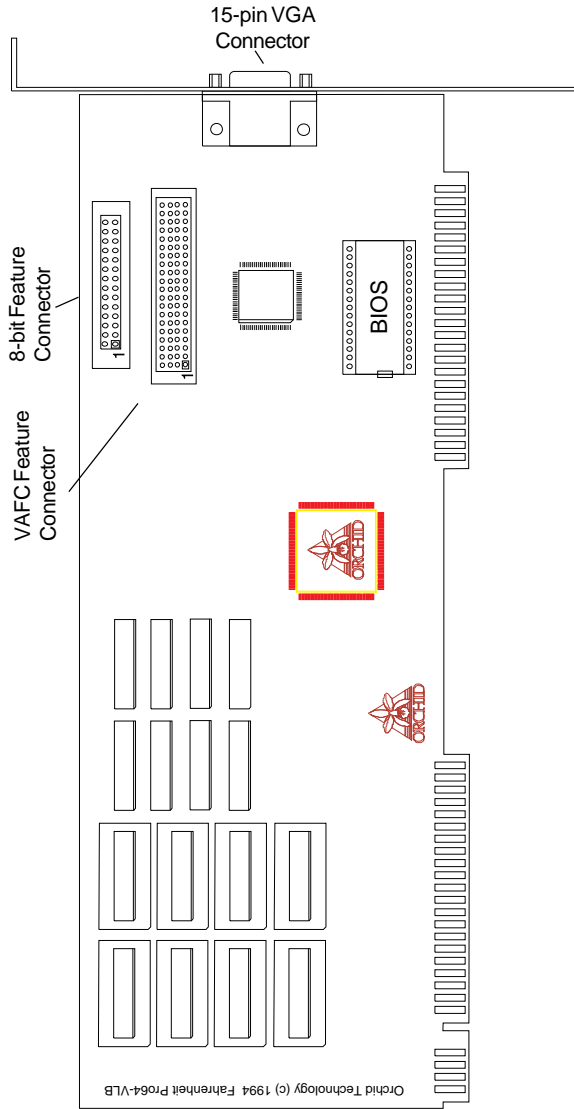
Figure 1.2: Fahrenheit ProVideo 64 VLB Diagram
