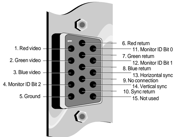
Figure A.1: Fahrenheit ProVideo 64 15-pin Connector
