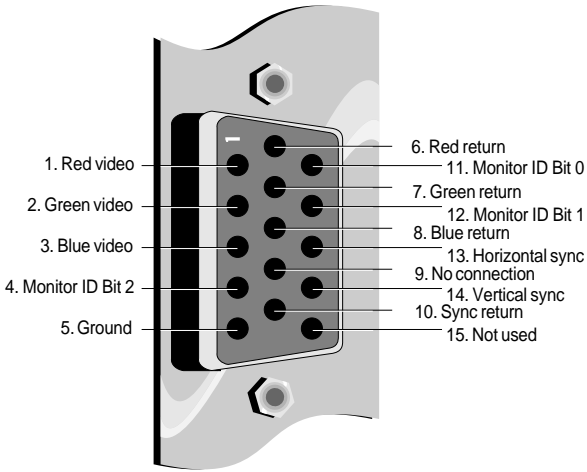
Figure 1.5: Standard 15 pin D-shell Connector
