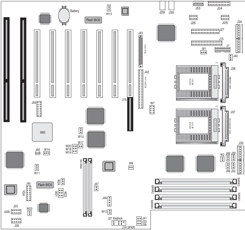
Figure 2.1: M6DPi System Board
