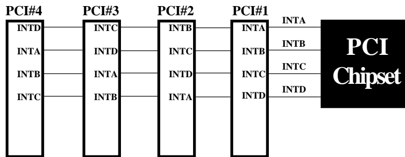
Figure 3-7 The Combination of PCI INT# lines
