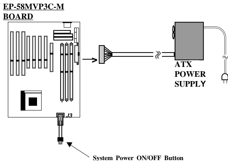
Figure 2-2: Simple ATX Power ON/OFF Controller
