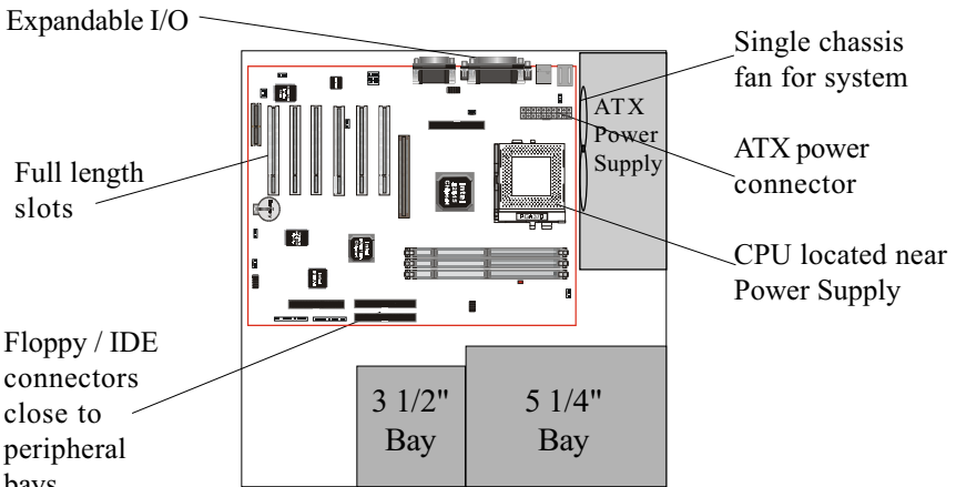
Figure 2: Summary of Micro-ATX chassis features
