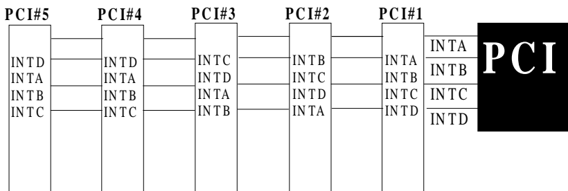
Figure 7: The Combination of PCI INT#lines
