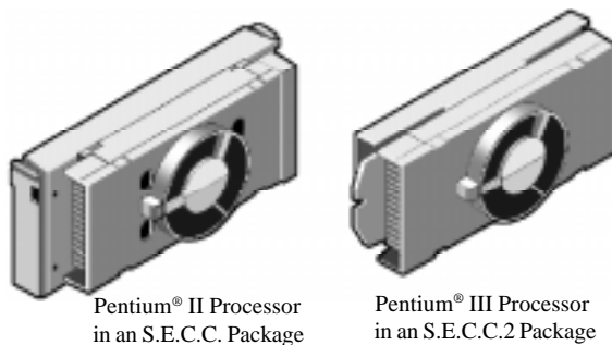
Figure 1: Pentium® II/III Processor CPU with S.E.C.C. or S.E.C.C.2 Package
