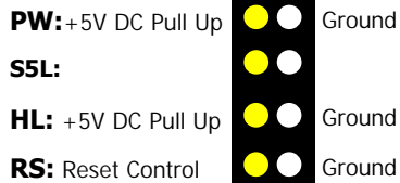
Top View of the System Panel and LED Connectors
