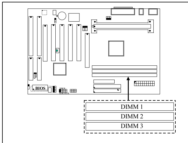
Picture of PT-6IBP DRAM subsystem
