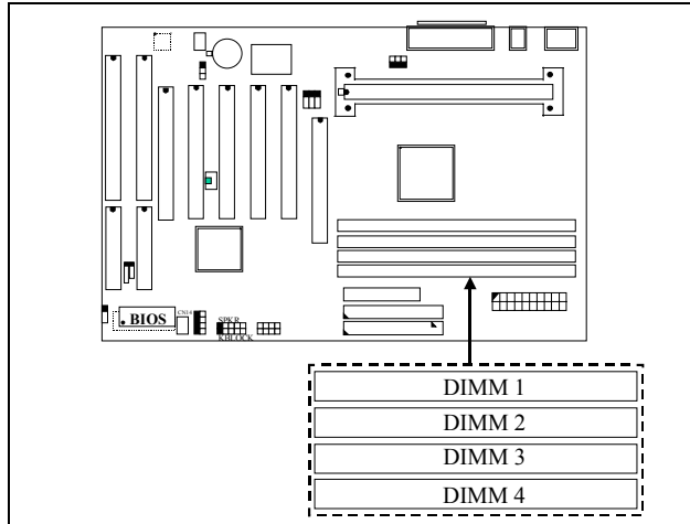
Picture of PT-6IBD DRAM subsystem
