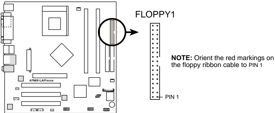
A7N8X-LA/Focus Floppy Disk Drive Connector
