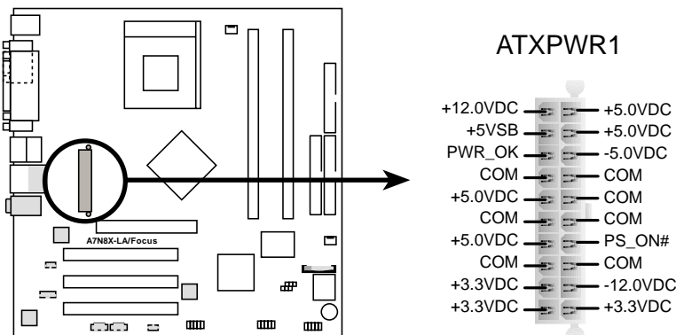
A7N8X-LA/Focus ATX Power Connector
