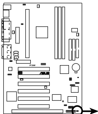
P3W IDE Activity LED
