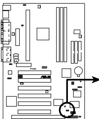
P3W Jumper Mode Setting
