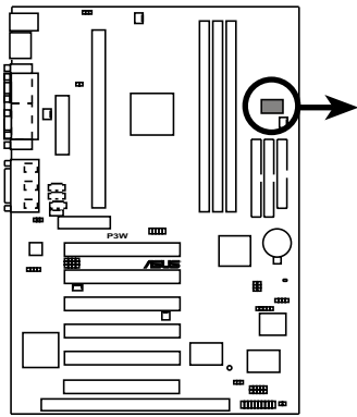
P3W DIP Switches
