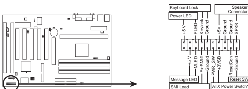
P2B-F System Panel Connections
