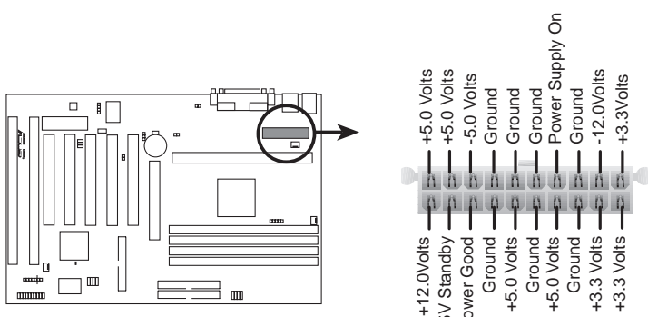
P2B-F ATX Power Connector
