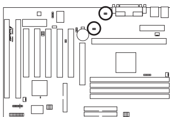
P2B-F Heat Sensor Connectors
